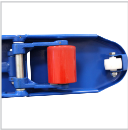
Entry rollers
